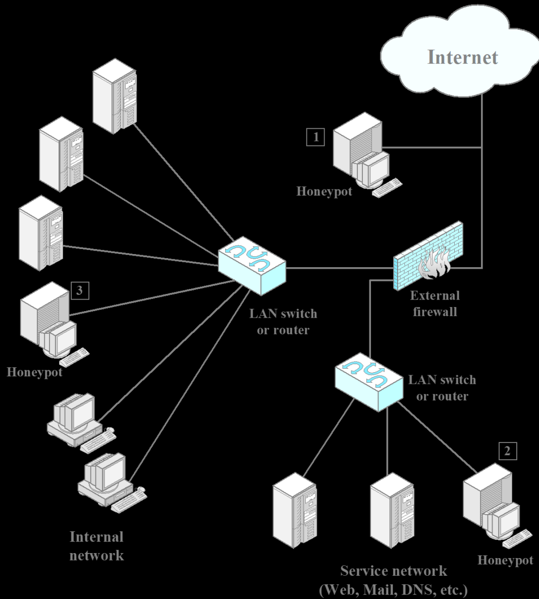
Figure 8.8 Example of Honeypot Deployment
